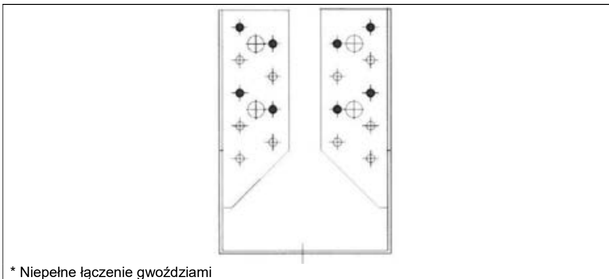
Rysunek 168 Typ WBZ 21, WBZ 23, WBZ 26
